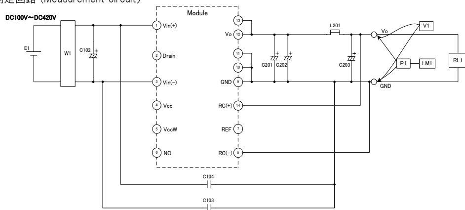
測定回路 (Measurement circuit)
