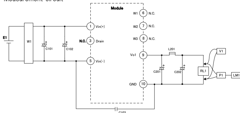
Measurement circuit
