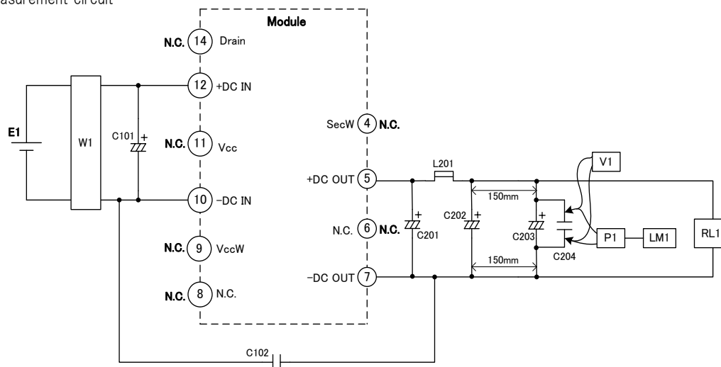
Measurement circuit
