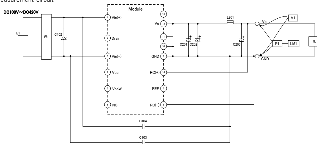
Measurement circuit
