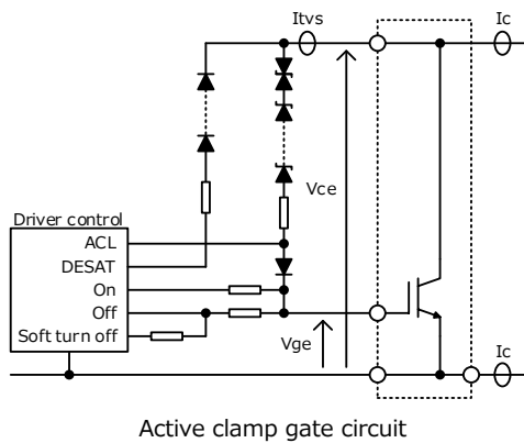
Active clamp gate circuit
