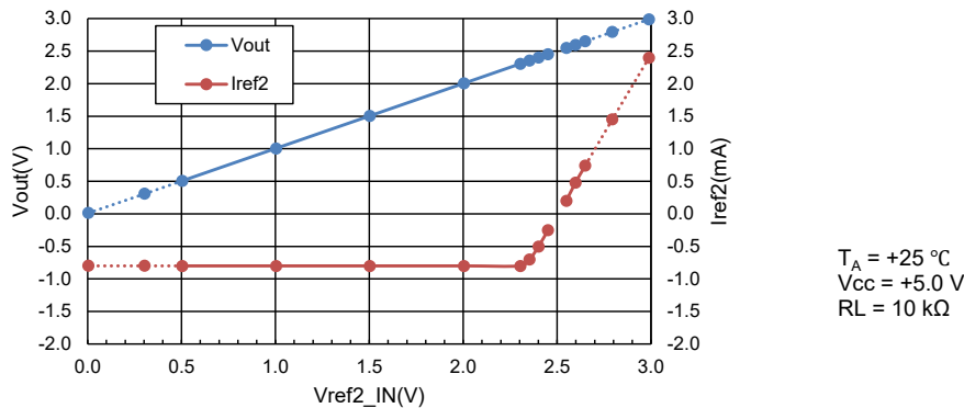
Fig 1 : Vref2 input voltage vs Output voltage and Iref2 (= Vref2 current) (Typical performance)
