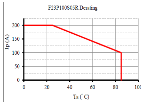
Figure 4: Ip vs Ta for F23P100S05R Measurement condition Vcc=+5V, RL=10kΩ
