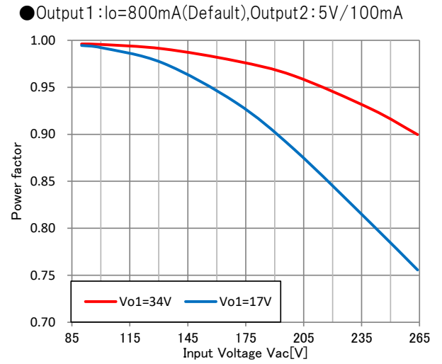
力率特性(Ta=25°C) Power factor characteristic
