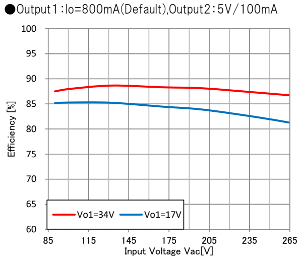
効率特性(Ta=25°C) Efficiency characteristic
