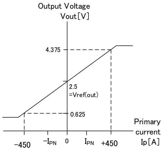
F26P150S12
